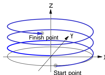
Fig. 3.3-2 Helical interpolation (one rotation or more)
