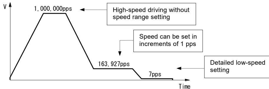
Fig. 1.1-7 Speed Range-Free
