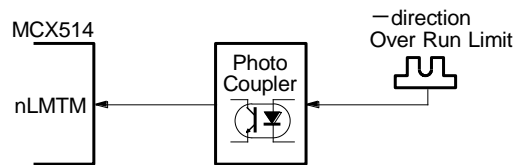
Fig. 2.5-15 Connection of Example 2 Automatic Home Search
