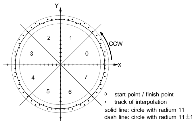
Fig. 3.2-3 Example of CircularInterpolation
