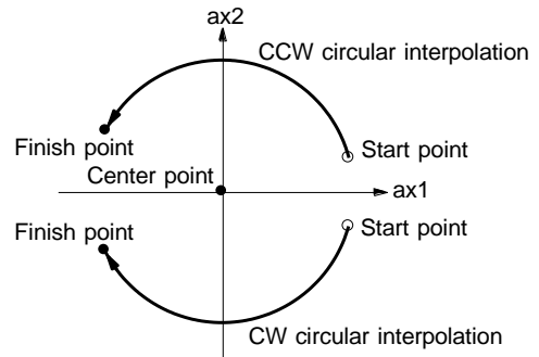
Fig. 3.2-1 CW/CCW circular interpolation
