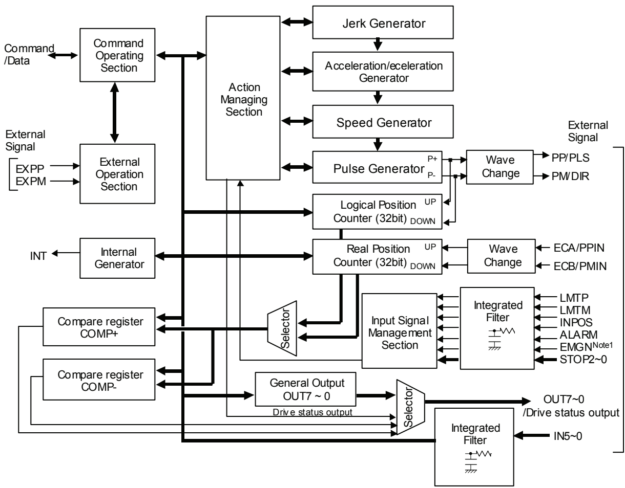
Fig. 1-2 Functional Block Diagram of Axis Control Section
