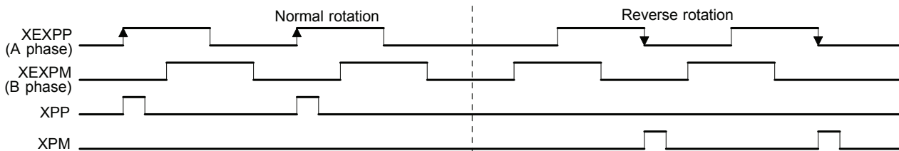
Fig. 2.27 Example Output Pulse 1 Driving by A MPG
