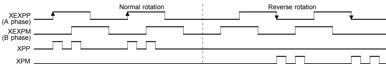
Fig. 2.28 Example of Output Pulse 2 Driving by A MPG
